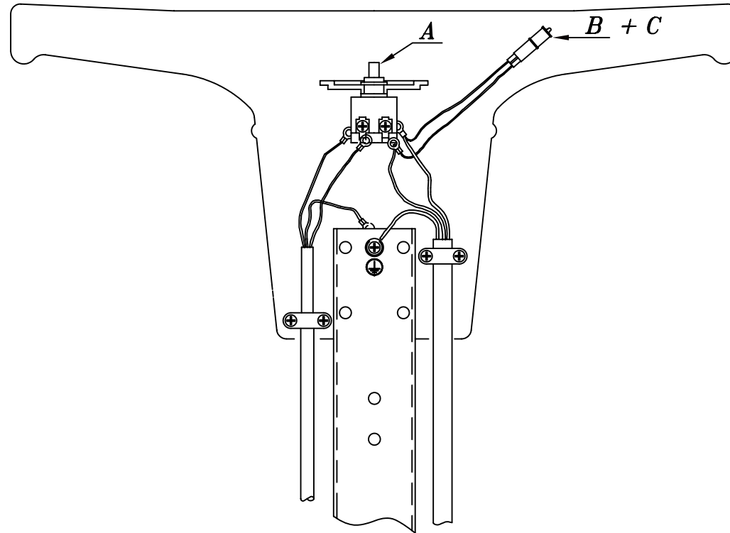
VIEW INSIDE HANDLE ASSY
