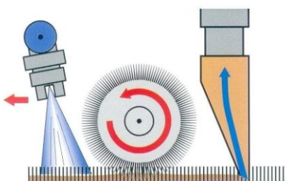
Injection-extraction cleaning with rotating brush
