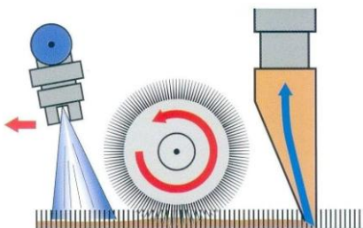
Injection-extraction cleaning with rotating brush
